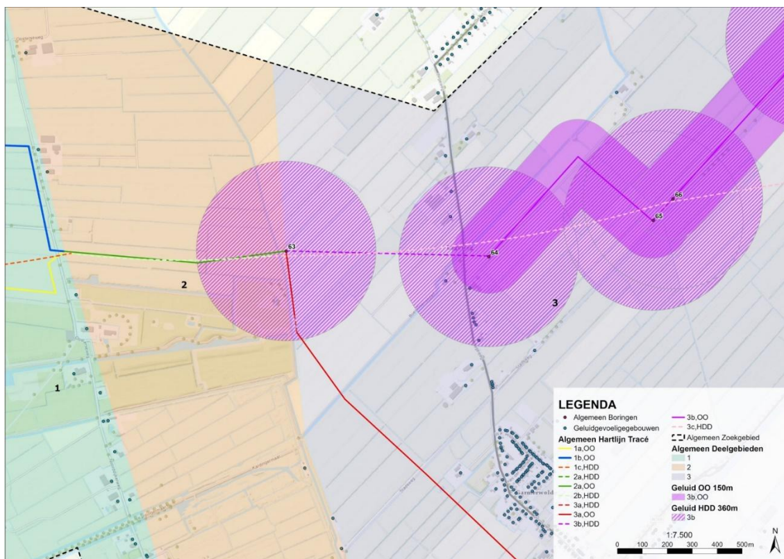
Figuur 8.14 Boring 63-64
