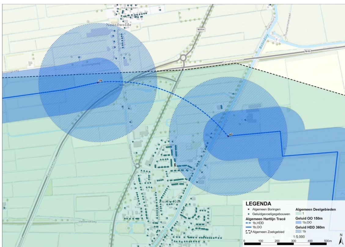
Figuur 8.6 Boring 39-40
