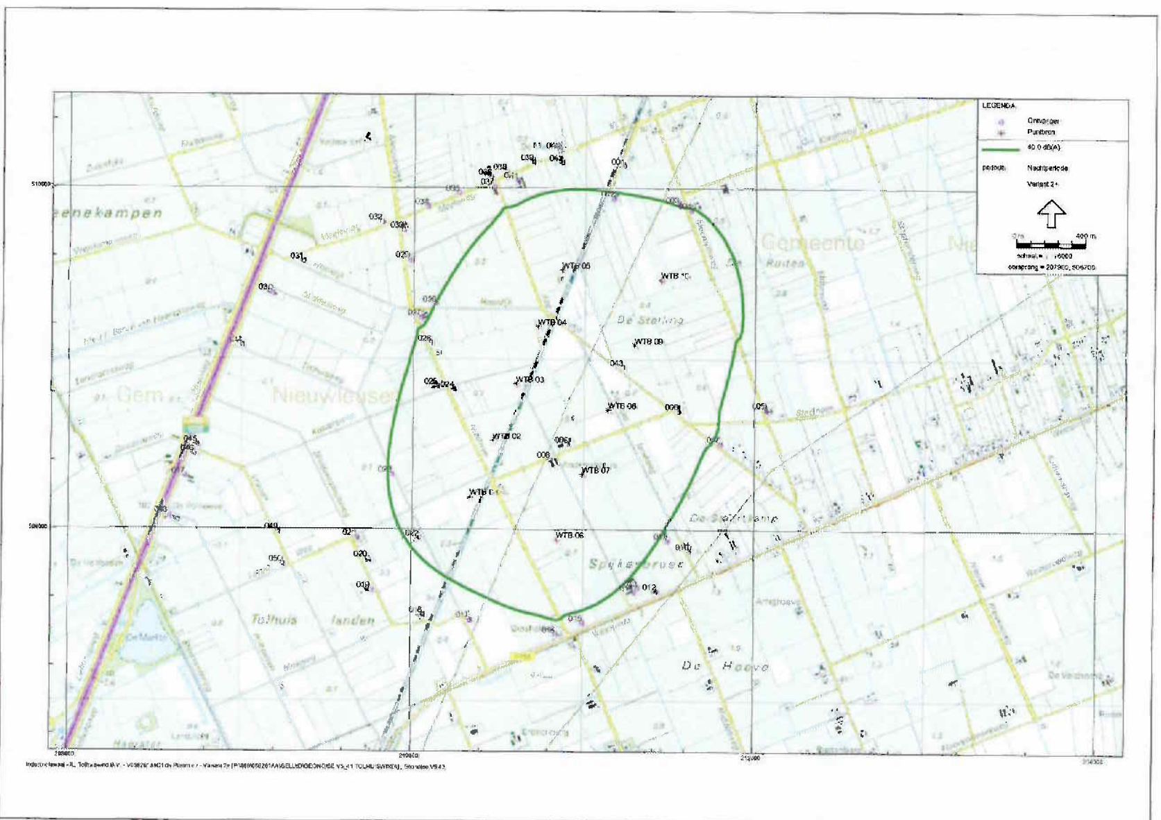
Figur 1.6 WNC-40 contour variant 2+
