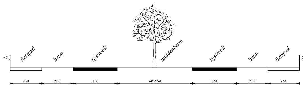
Principeprofiel centrale as
